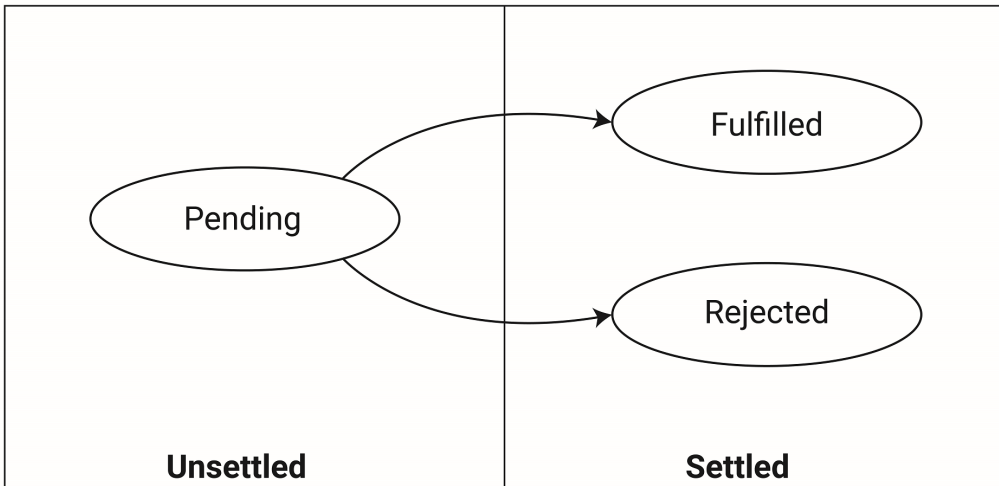
Figure 1-1: Promise states
